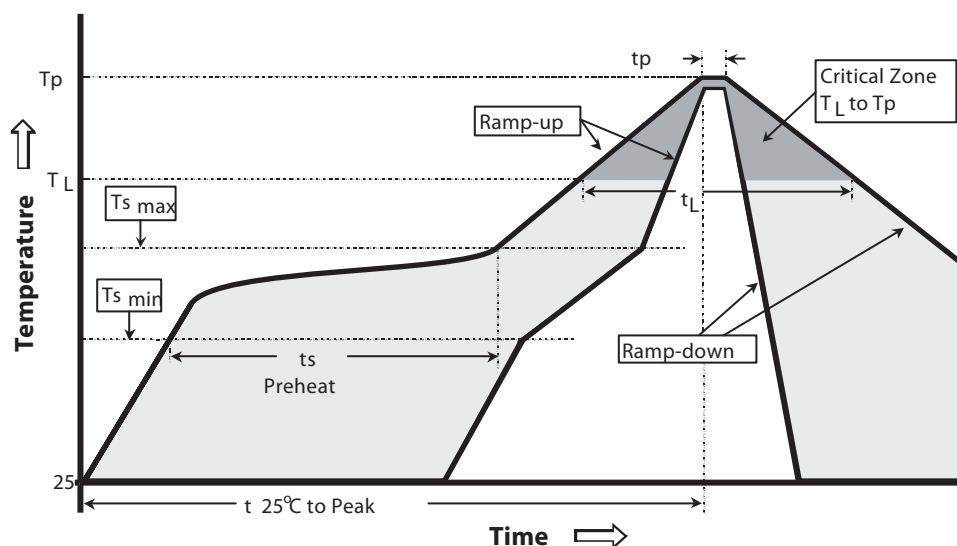
Figure 23. Typical SMT Reflow Profile for Maximum Temperature = 260 +0/-5^{\circ}\text{C}
